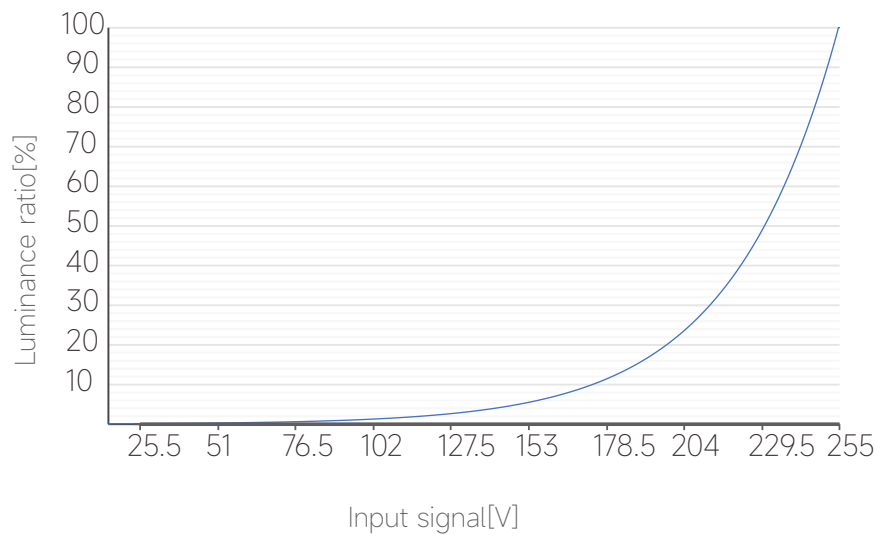
The AIDimming developed dimming curve
